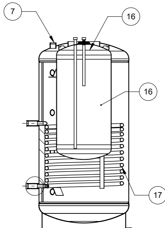
SECTION B-B
