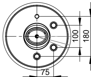
DETAIL H SCALE 1 : 10
